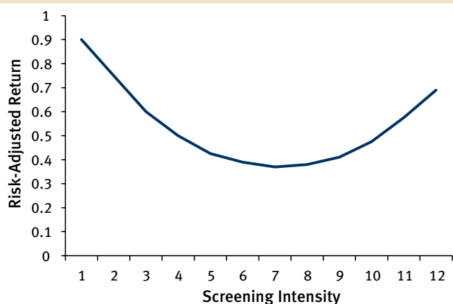
Relationship Between Return and Screening Intensity
